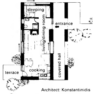
⑧ Holiday house in Greece
